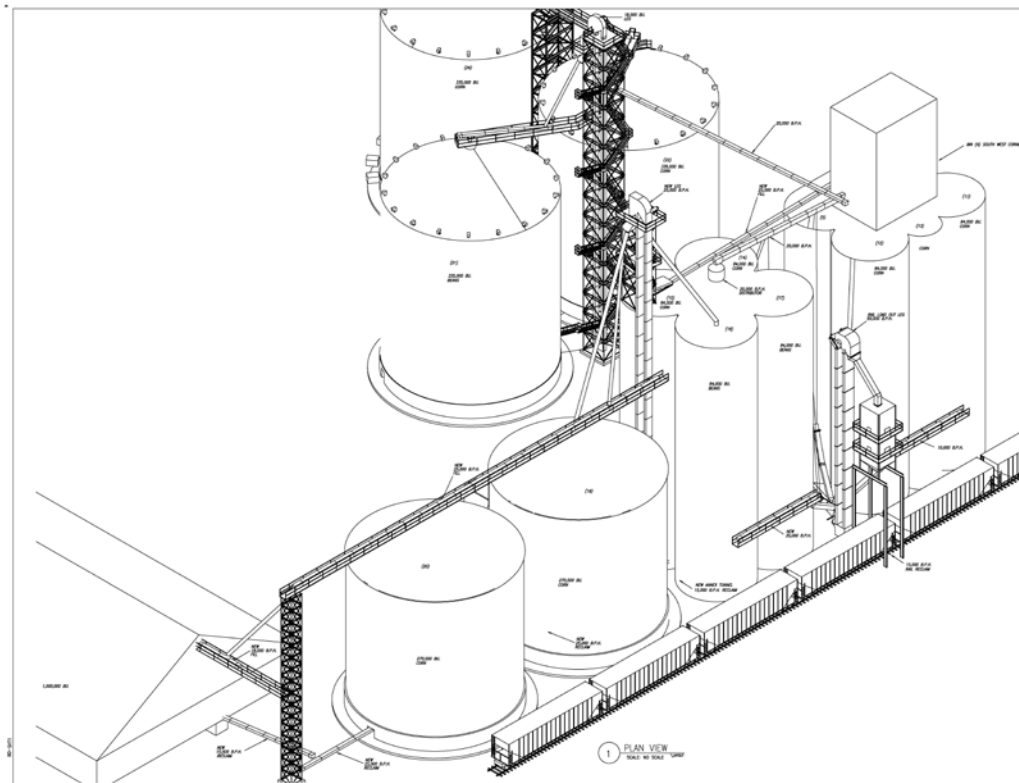
3D Project layout Model
