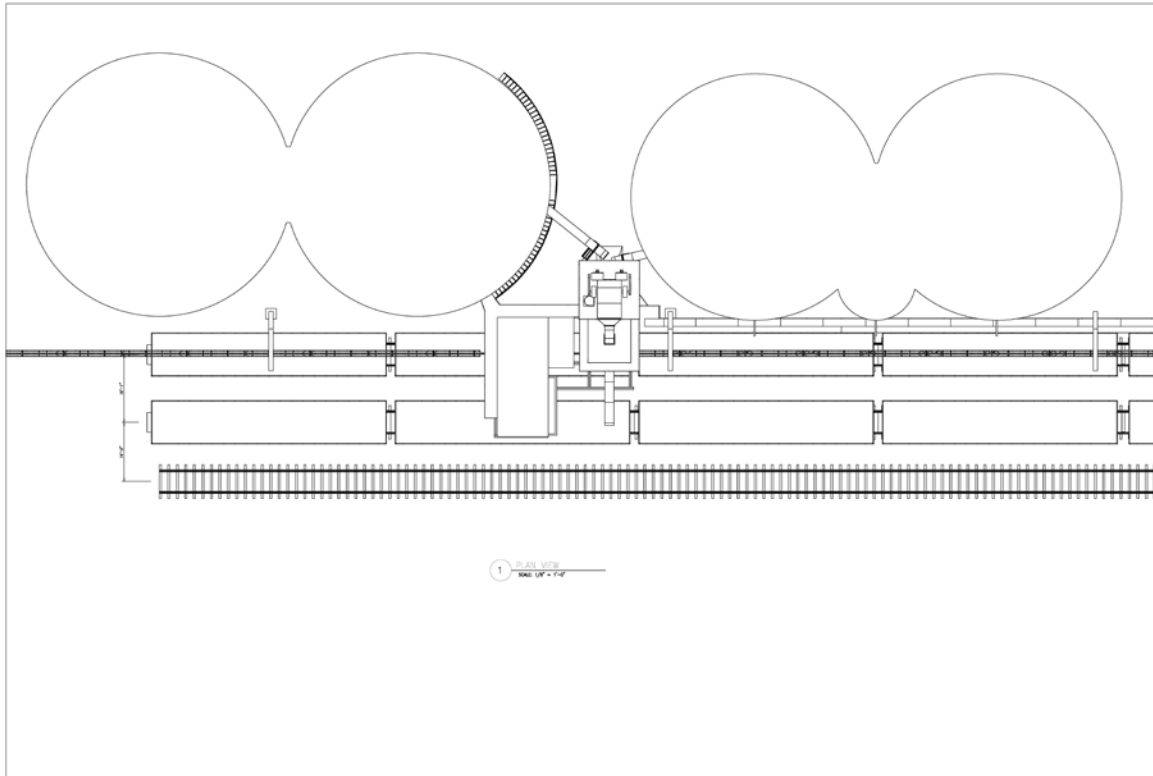
Preliminary Layout Plan
