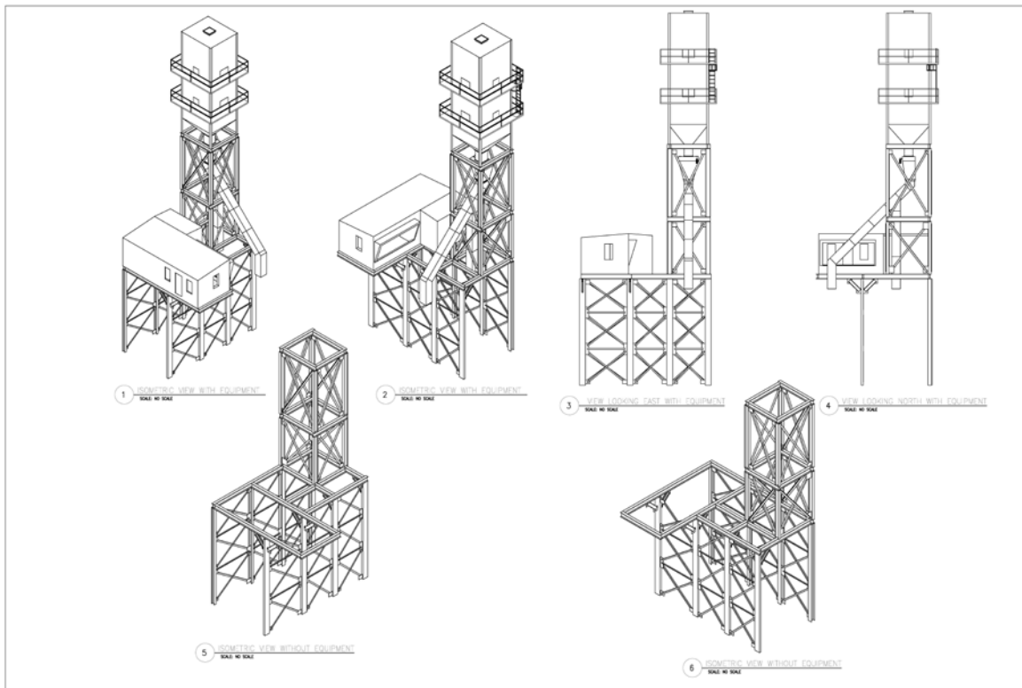
3D Bulk Weigher Support Structure model
