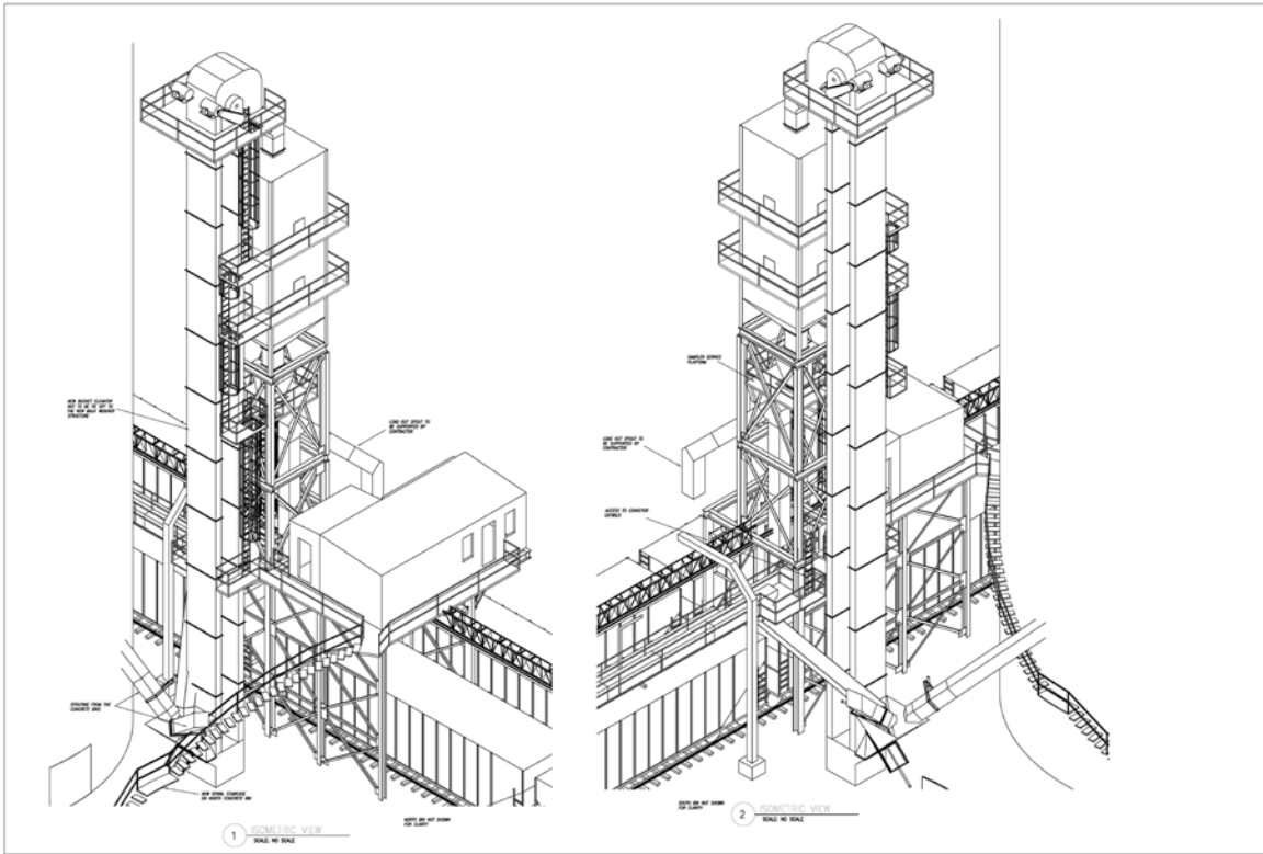
3D Project Layout Model
